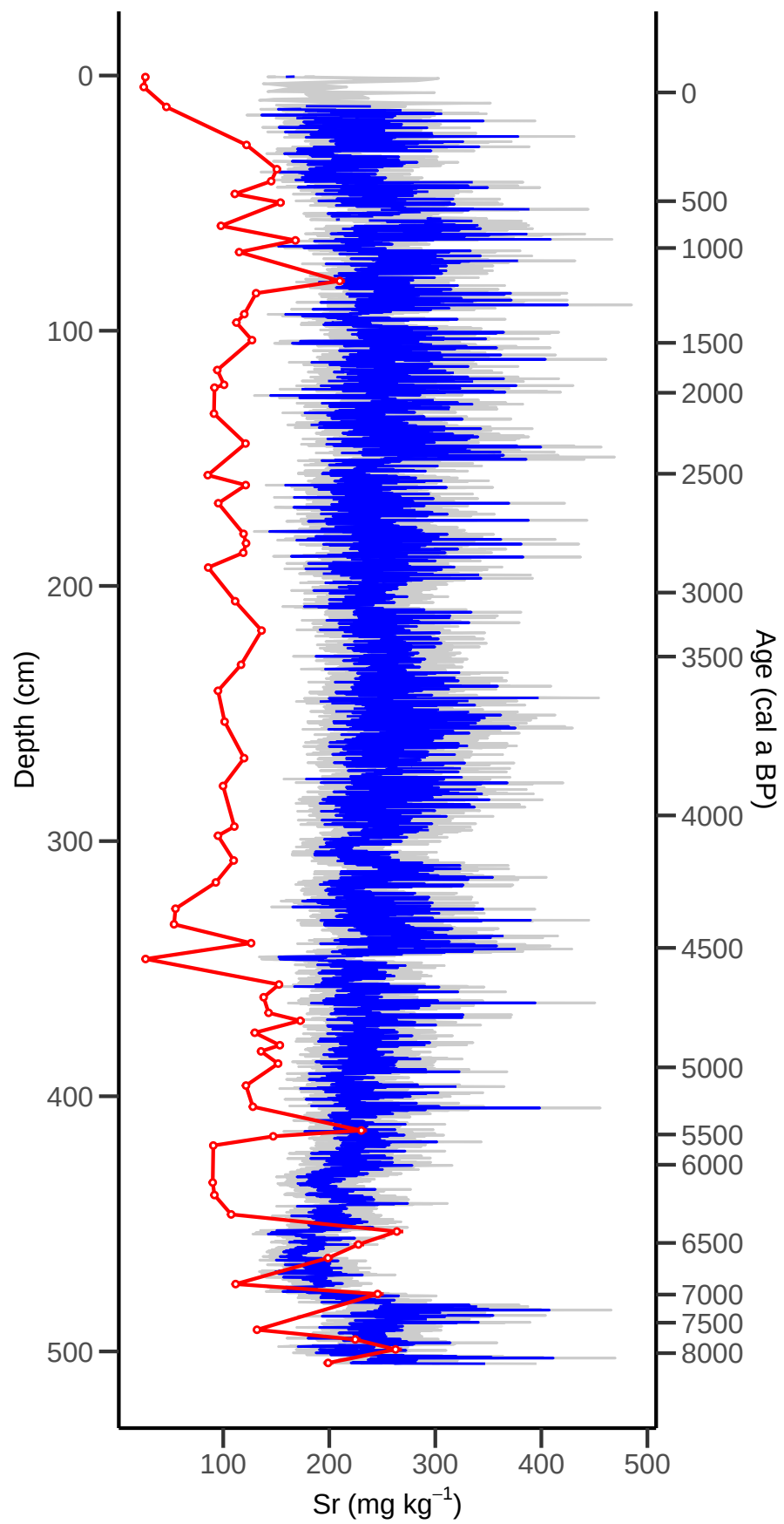
BI10: PLSR Sr Predictions with Confidence Intervals
